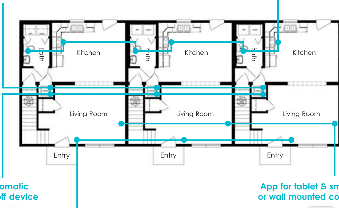
Motion Sensor
